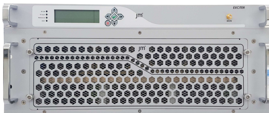
900W Air Cooled DTV Transmitter (483 x 198.5 x 631mm)
