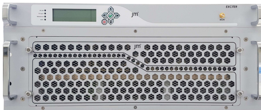
600W Air Cooled DTV Transmitter (482 x 200 x 630mm)
